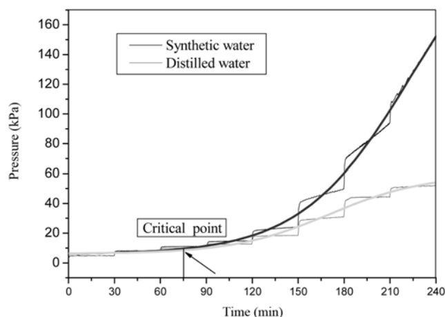
Fig. 2. Critical flux determination by the flux-steps method.
